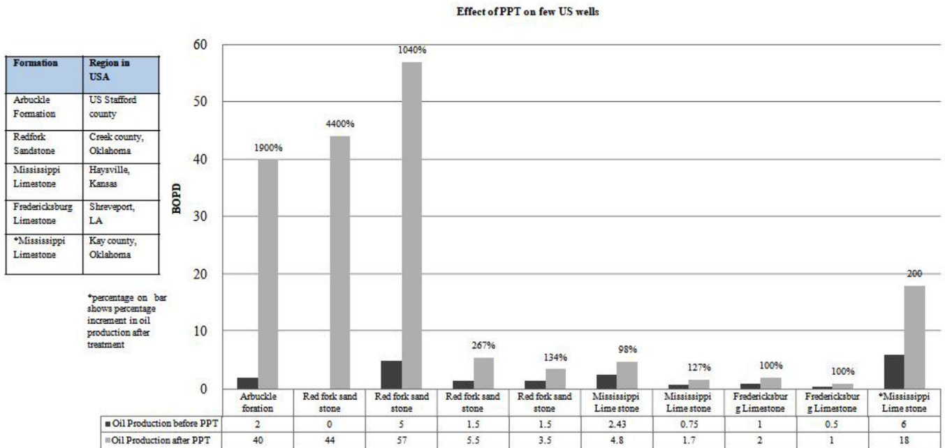
Fig. 8. Effect of PPT on oil production from sandstone and limestone formations of few US fields. 4
