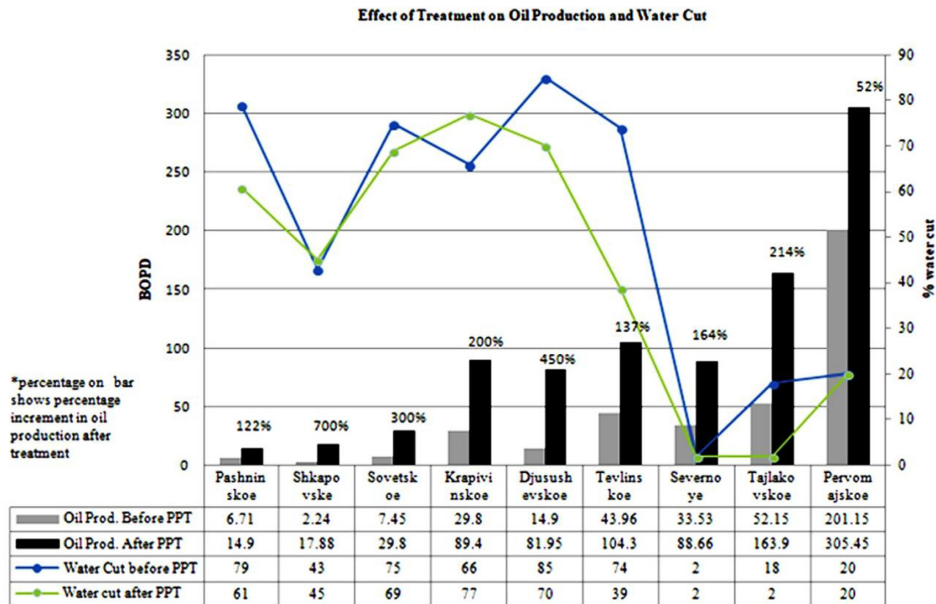
Fig. 7. Oil production and % water cut before and after of PPT treatment on production well of few oil fields of Russia (data from Novas Energy, 2015). 2
