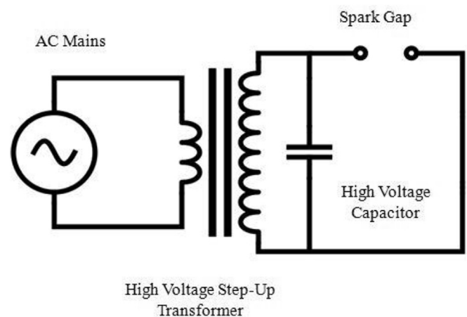
Fig. 5. Simple electric circuit diagram showing formation of plasma arc across spark plug.
