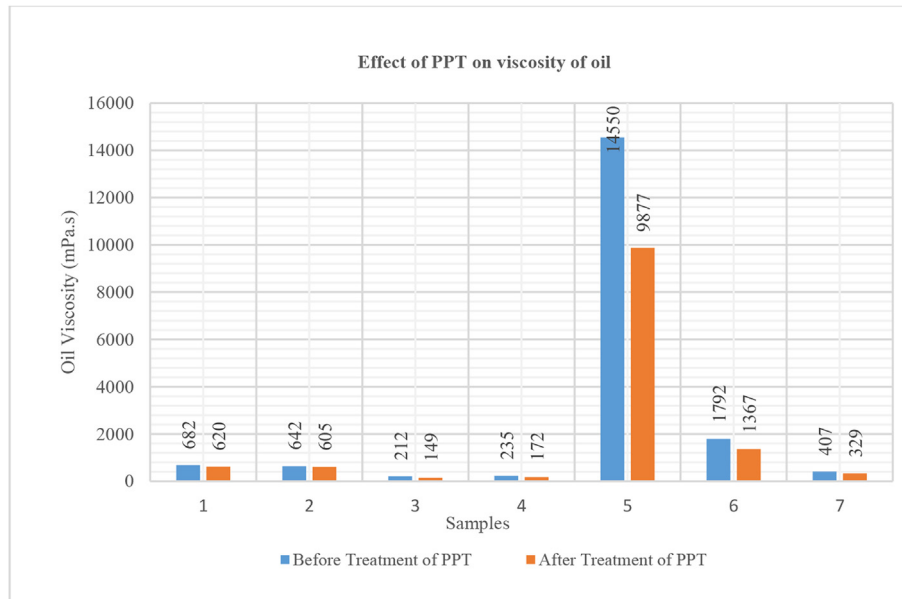
Fig. 6. Reduction in effective viscosity observed after application of PPT (modified after Maksyutin and Khusainov, 2014).
