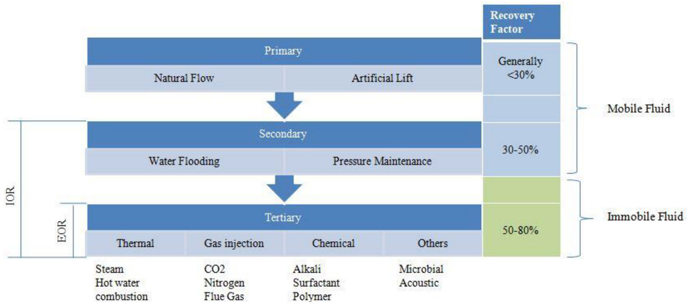
Fig. 1. Defining improved oil recovery (IOR) and enhanced oil recovery (EOR) (Stosur et al., 2003).
