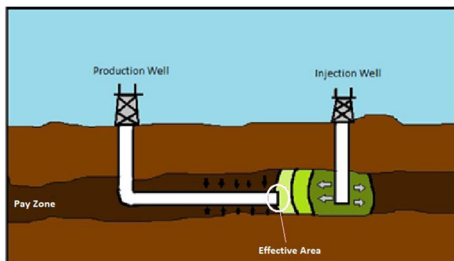
Fig. 2. Illustrative diagram showing EOR treatment being applied to horizontal well and ineffectiveness of EOR method due small effective area of producing well being treated.
